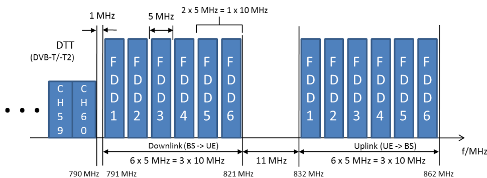
Figure X Illustration of “800MHz” LTE mobile communication network services frequency use (3GPP band 20)
