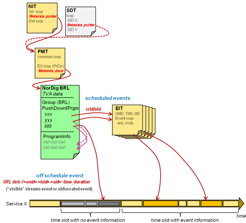
Figure 6 Signalling model for NorDig Broadcast Record List (BRL).
