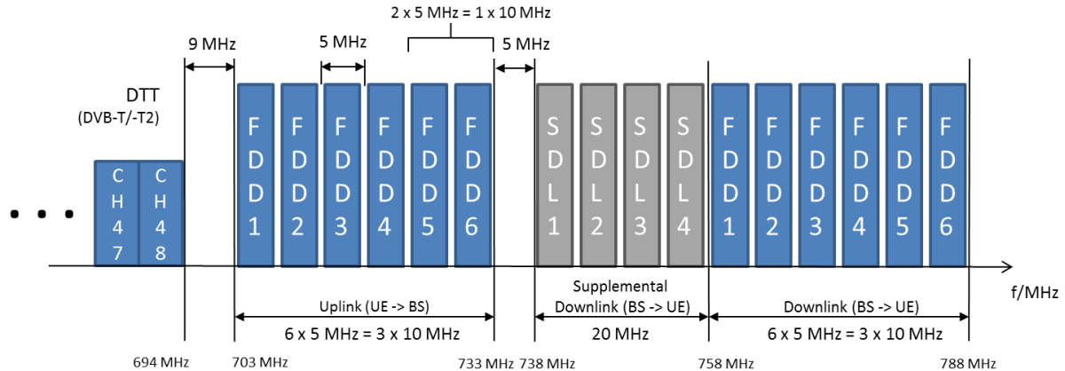
Figure Y Illustration of "700MHz" LTE mobile communication network services frequency use (3GPP band 28a plus Supplemental Downlink band)
