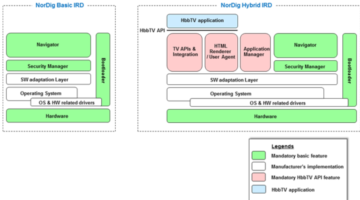
Figure 2.3: Possible software architecture of a NorDig , to the left a NorDig Basic IRD without NorDig API and to the right a NorDig Hybrid IRD with NorDig API (i.e. HbbTV API).
