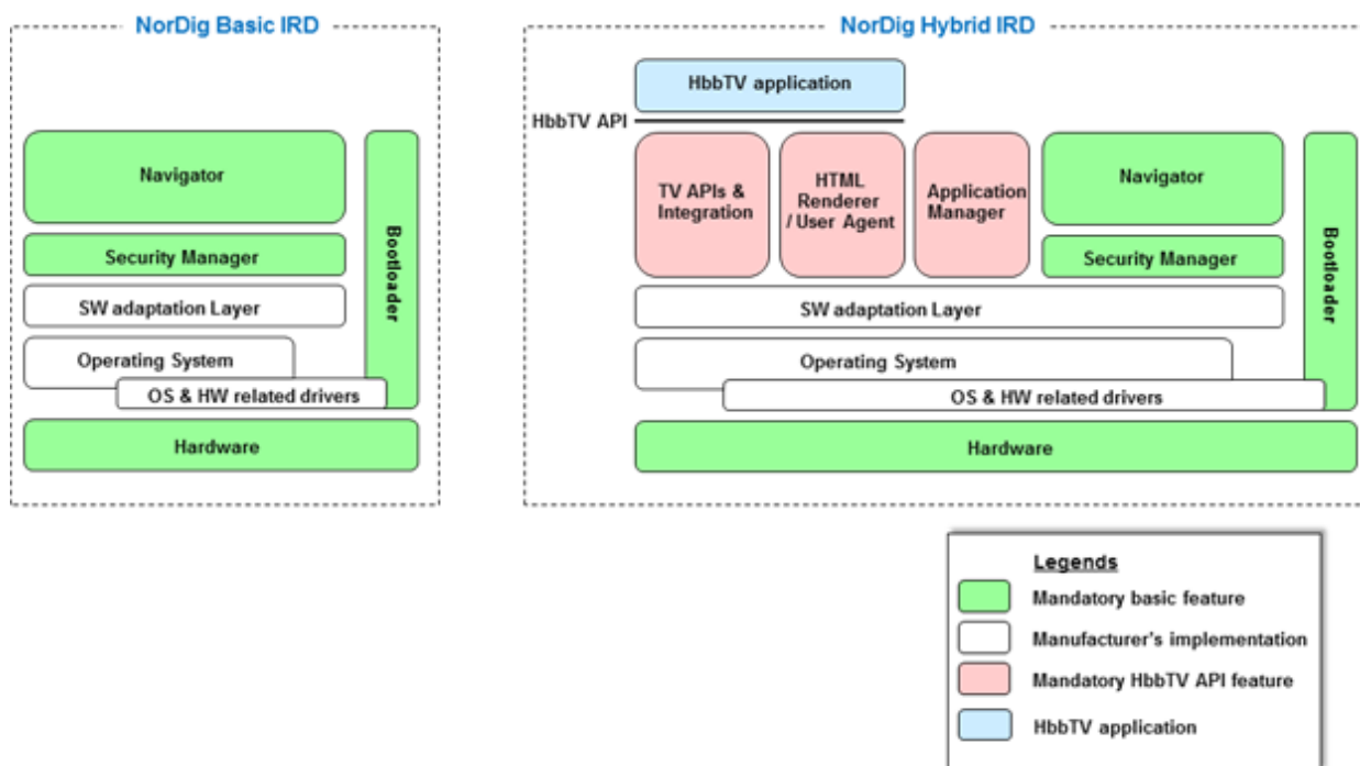
Figure 2.3: Possible software architecture of a NorDig, to the left a NorDig Basic IRD without NorDig API and to the right a NorDig HbbTV IRD with NorDig API (i.e. HbbTV API).
