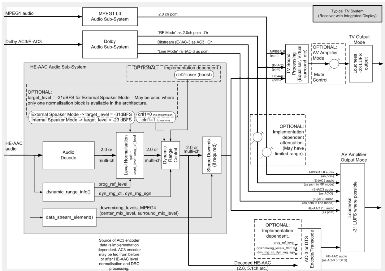
Figure Annex H 1: Loudness levels – Typical IDTV Audio Block diagram.
