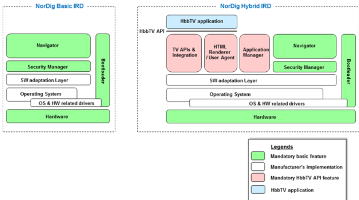
Figure 2.4: Possible software architecture of a NorDig, to the left a NorDig Basic IRD without NorDig API and to the right a NorDig HbbTV IRD with NorDig API (i.e. HbbTV API).
