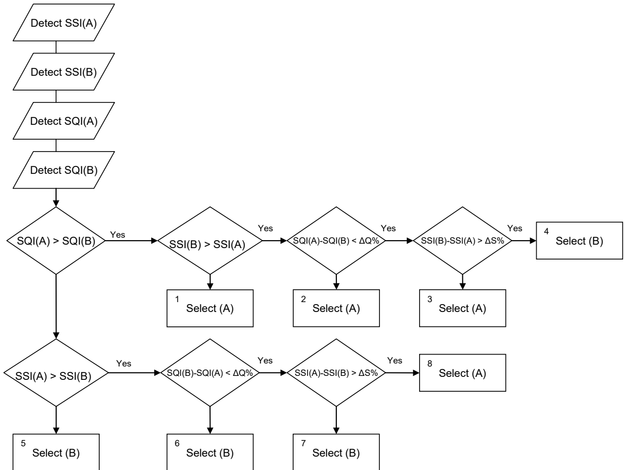
Figure 1: A flowchart for best service selection algorithm in case when two transmitters A and B transmit equal service and both of them are able to be received. \Delta S and \Delta Q refer to difference in SSI and SQI values and are defined as \Delta S=10\% and \Delta Q=20\% .
