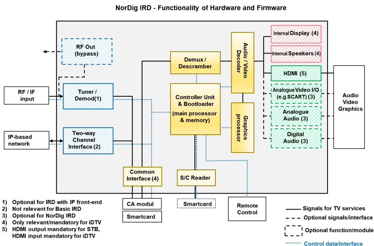
Figure 2.2 Functionality of Hardware and Firmware for NorDig IRD
